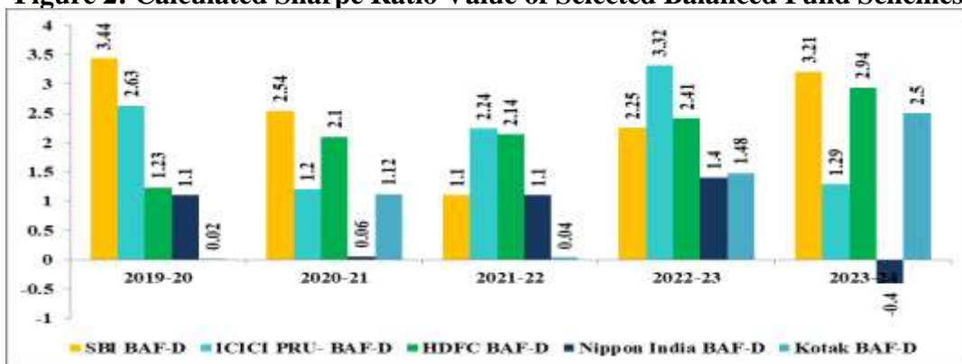
Figure 2: Calculated Sharpe Ratio Value of Selected Balanced Fund Schemes
