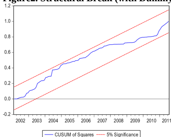
Figure2. Structural Break (with Dummy Variable)
