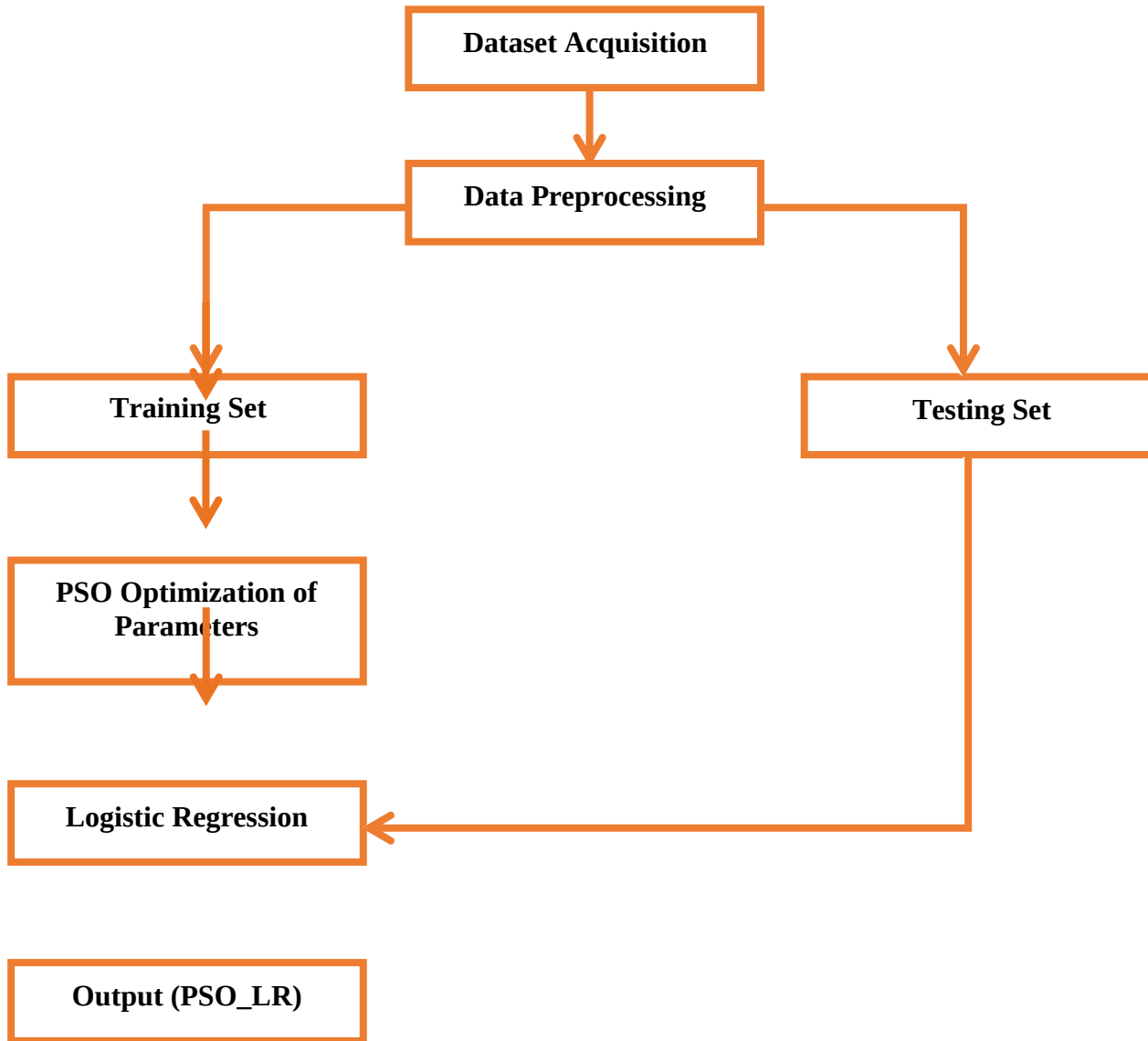
Fig 3.5: PSO-LR Flowchart
