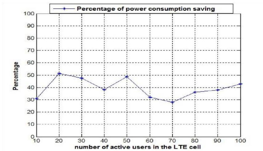
Fig. 7. Percentage of Power Consumption saving.
