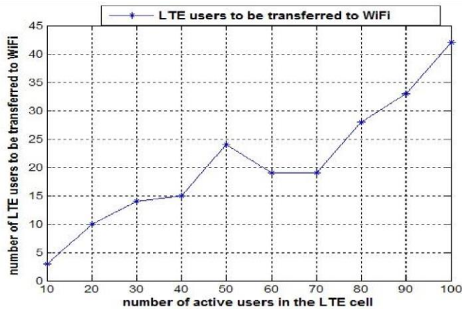
Fig. 2. Number of users to be offloaded to WiFi with respect to the total number of active users in the LTE cell. Taking into consideration that the LTE users will be offloaded when their demands exceed the 20 Mbps, considered as the average per user throughput in LTE-A network [11], the minimum needed number of WiFi APs, and the acquired throughput in the WiFi network are shown in Fig. 3 and Fig. 4 respectively, noting that there is no restriction in this case on the maximum offered throughput per user in the WiFi network.
