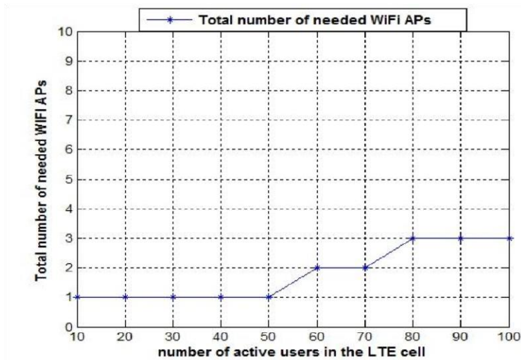
Fig. 5. Total number of needed WiFi APs with average per user WiFi throughput set to 20 Mbps maximum. To pinpoint the saving in LTE when applying our proposed dimensioning method, we have measured the average power consumption saving related to the transmitted power after being transferred to WiFi. Fig. 6 and Fig. 7 represent the average saved power consumption in the eNB in Watts, and the percentage of power saving in respect to the total consumed power, respectively. As we can observe, there is on average 40% saving of the total consumed power in the eNB. This saving is expected to grow obviously when the number of offloaded users increase.
