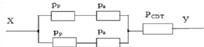
Figure 2. RBD of two-channel RCPU with two equally reliable SW versions (their PF p_p(t) ) and equally reliable channels HW (whose PF p_a(t) ) (St1)
