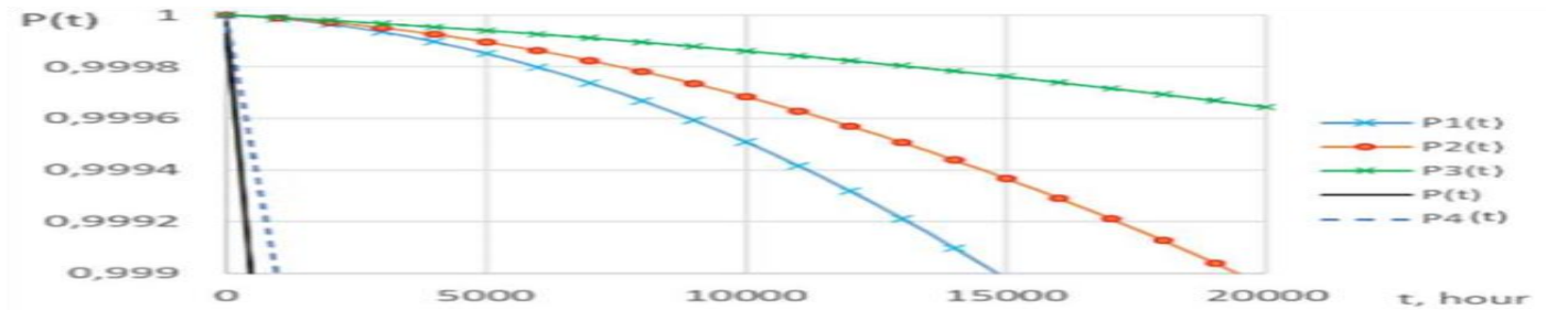
Figure 8. Graphical dependencies of PF structures RCPU St0, St1, St2, St3, St4 on time until the failure \lambda_a = 10^{-6} 1/h, \lambda_p=10^{-6} 1/h, \lambda_{a1}=10^{-7} 1/h, \lambda_{p1}=10^{-7} 1/h, \lambda_{CDT}=10^{-8} 1/h.
