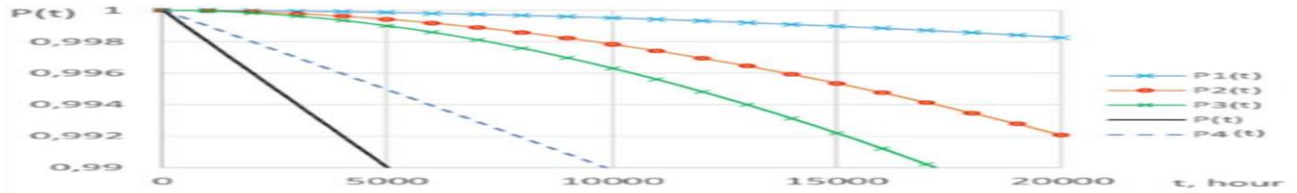
Figure 6. Graphical dependencies of PF structures RCPU St0, St1, St2, St3, St4 on time until the failure \lambda_a=10^{-6} 1/h, \lambda_p=10^{-6} 1/h, \lambda_{a1}=10^{-5} 1/h, \lambda_{p1}=10^{-5} 1/h, \lambda_{CDT}=10^{-8} 1/h.
