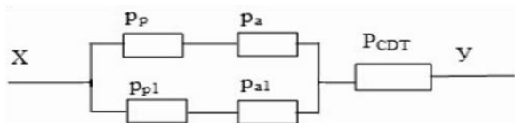
Figure 4. RBD of two-channel RCPU with two not equally reliable SW versions and HW channels (St3).
