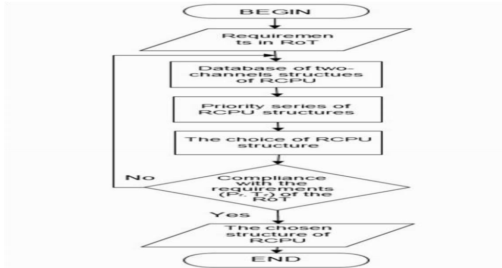
Figure 15. An algorithm for selecting of RCPU structures based on the formation of priority series, where P_r is the PF
