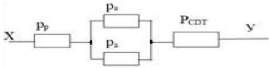
Figure 5. RBD of two-channel RCPU with one SW version
