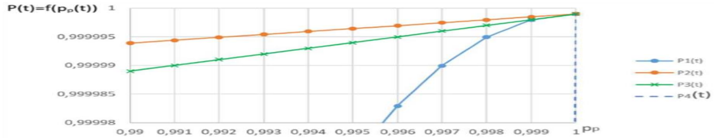
Figure 14. Graphs of the dependence (a, b) of the PF of RCPU structures St1, St2, St3, St4 on the PF of the SW of the first (main) channel if p_a(t)=0,99999 ; p_{a1}(t)=0,9995 ; p_{p1}(t)=0,9995 ; P_{CDT}(t)=0,999999 .
