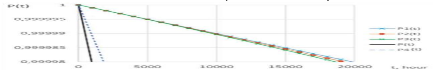
Figure 9. Graphical dependencies of PF structures RCPU St0, St1, St2, St3, St4 on time until the failure \lambda_a = 10^{-8} 1/h, \lambda_p=10^{-8} 1/h, \lambda_{a1}=10^{-7} 1/h, \lambda_{p1}=10^{-7} 1/h, \lambda_{CDT}=10^{-9} 1/h. The interest is the study of how impacts on PF of RCPU structures PF of the first (main channel) SW version (Fig. 10-14).
