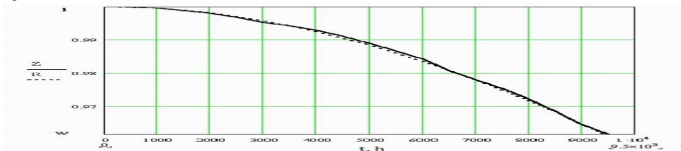
Figure 16. Graph of the dependence of the PF reserved HW and two-versions RCPU on time, obtained using imitation simulation (Z) and analytical (R) modeling under the Condition of exponential distribution of the failure flow of HW and SW and St4 architecture.
