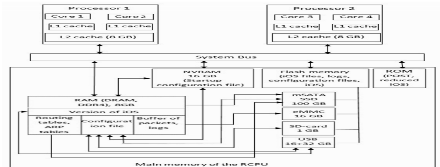
Figure 1. The main locations of SW in N-version programming in different types of memories.
