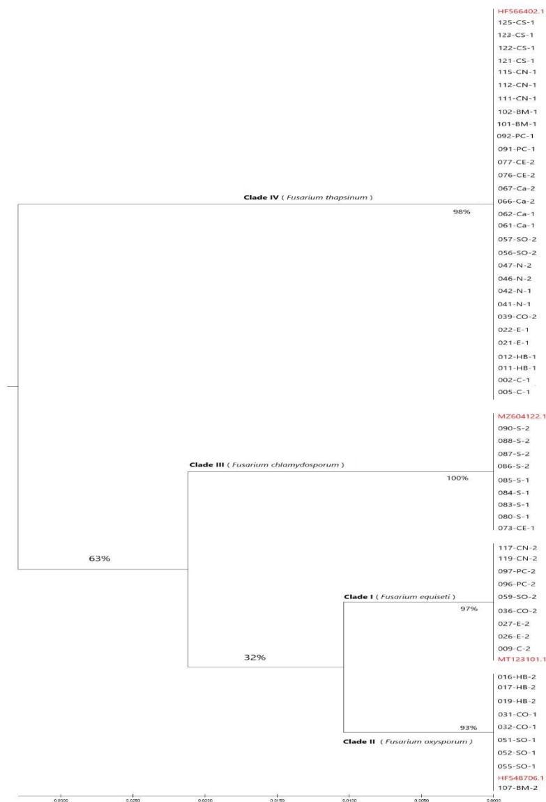
Fig. 3. Phylogenetic tree generated using nucleotide sequence information from the ITS region of conserved ribosomal DNA of Fusarium isolates.
