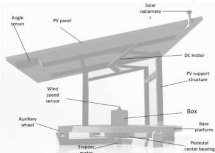
Figure 2: Three dimensional view of device body
