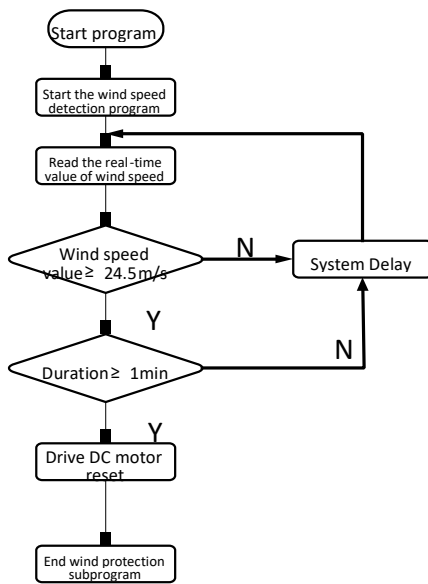
Figure 4: Flow chart of wind protection subprogram
