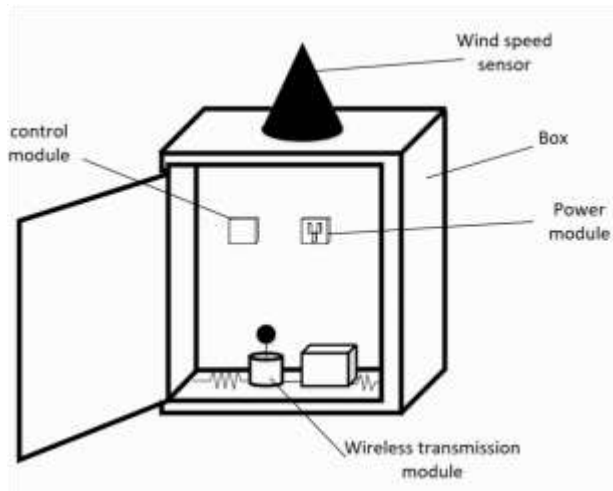
Figure 3: Internal Composition of Box
