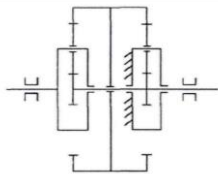
Figure 1: Planet carrier input + sun gear output
