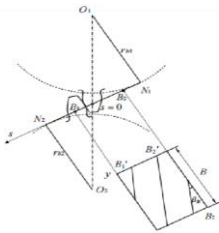
Figure 1: Example Diagram of Helical Gear Engagement
