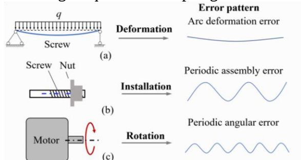
(a) Positioning error attributed to deformation forced by gravity (b) Assembly error of screw-nut pair (c) Rotational deviation of motor.
