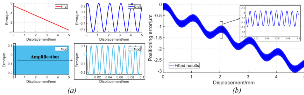
Figure 17: (a) The error pattern of predicting positioning errors in the BMS (b) The calculated predicting positioning errors in the BMS.
