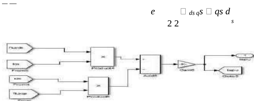
Figure 8: Torque estimator Simulink block
