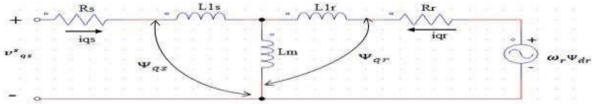
Figure 2: Equivalent circuit in quadrature axes referred to the stationary reference frame
