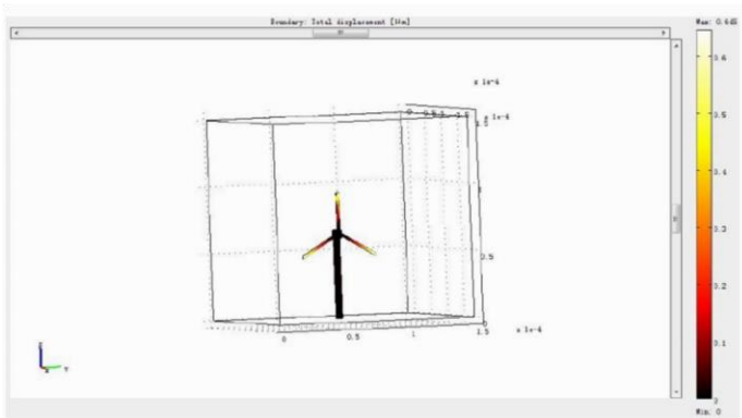
Figure 10 Total displacement in 1.5m/s maximum inlet speed in Case 1
