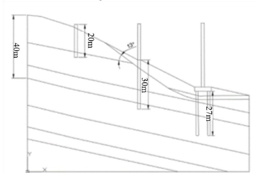
Figure 1: Calculation model of zhangyoufang Bridge
