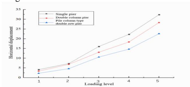
Figure 9: Horizontal displacement of various structural forms of pier 0
