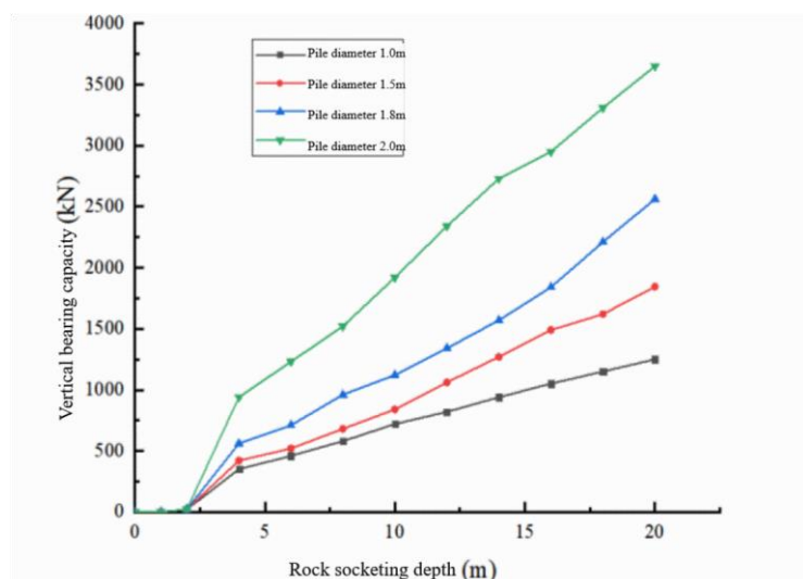
Figure 5: Distribution of vertical bearing capacity of different pile diameters
