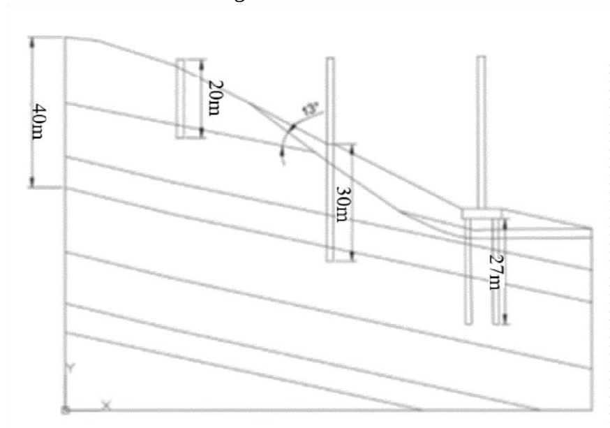
Figure 1: Calculation model of zhangyoufang Bridge
