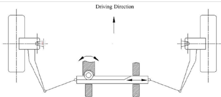
Figure. 1 Rear-displacement steering trapezoidal structure intention of the steering gear behind the front axle
