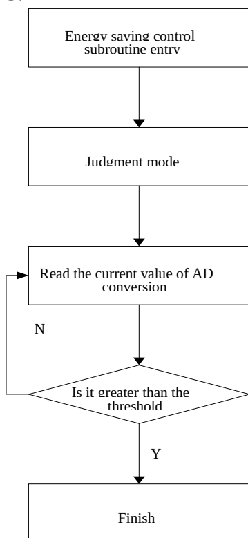
Figure 3. Energy saving control subroutine flowchart
