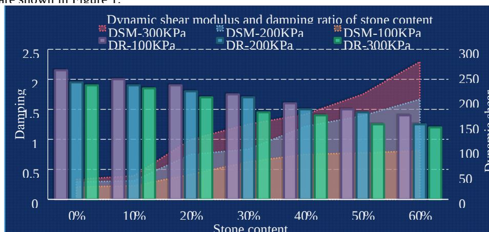
Figure 1. Changes of dynamic shear modulus and damping ratio in different contents of rock
