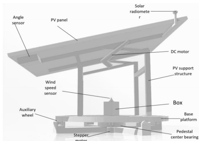
Figure 2: Three dimensional view of device body
