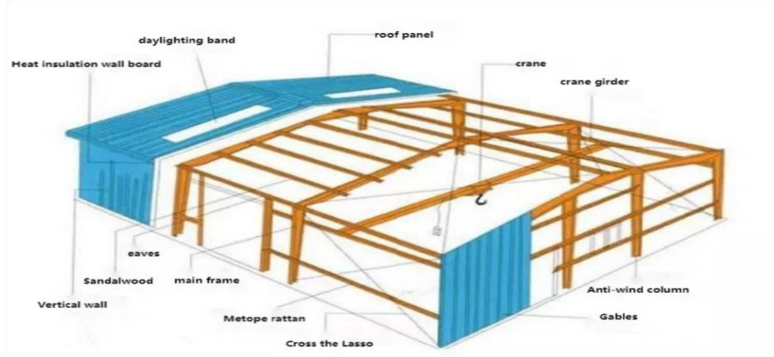
Figure 1: Construction technology of light steel structure roof purlin of portal steel frame
