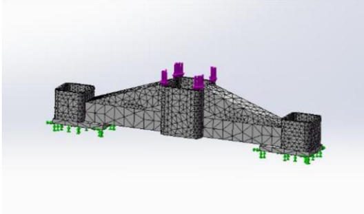
Figure 11: Schematic diagram of grid division of positioning displacement platform
