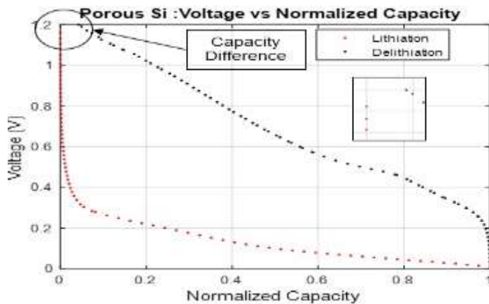
Figure 1a. Voltage vs Normalized Capacity before Side Reaction Correction. Red dots indicate Lithiation and Black dots denote delithiation.
