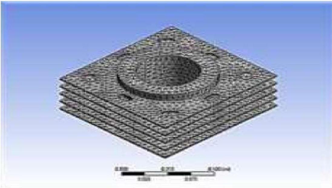
Figure 7. Mesh model of rectangular fin with slots.
