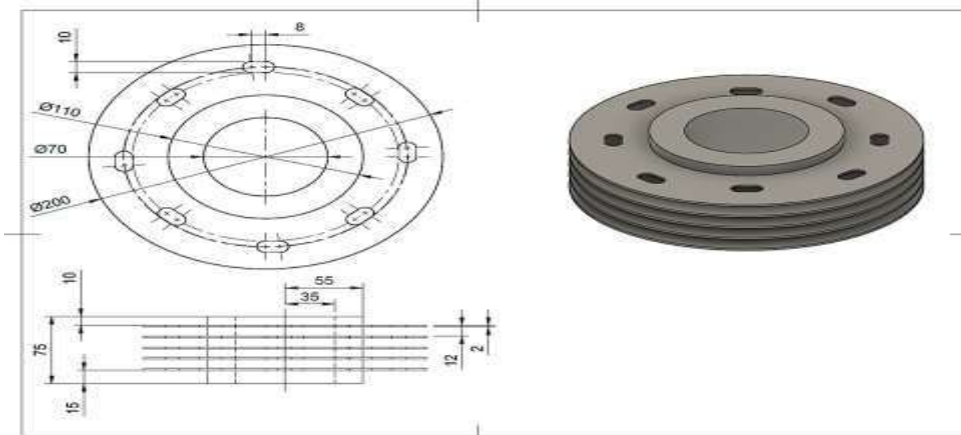
Figure 4. Circular fin model of 2 mm thickness with slots.
