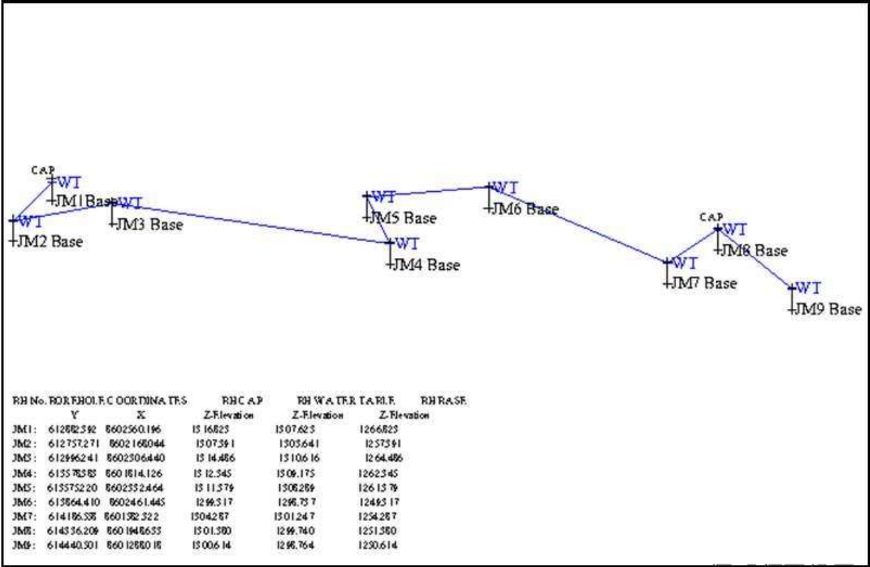
Figure 3: Plot of boreholes in space – Base and cap elevations (generated by Surpac) The resulting information was then used to estimate gradient between boreholes and this information was used to determine the follow direction. Figure 4 shows the contour plots of the water table and the gradient between boreholes and water flow direction (as constructed) from the gradients.
